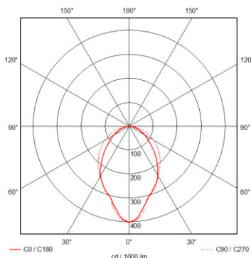
Polar curve – ASR 2x14w
